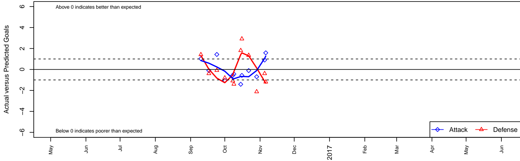
KVJSA Ellensburg FC B06 Dots are actual minus expected GF (blue circles) and GA (red triangles). Blue line is smoothed change in attack strength. Red is smoothed change in defense strength.
